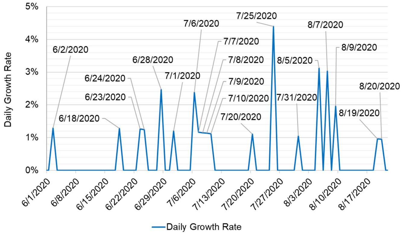
Daily Growth Rate - June 1, 2020 to Present
