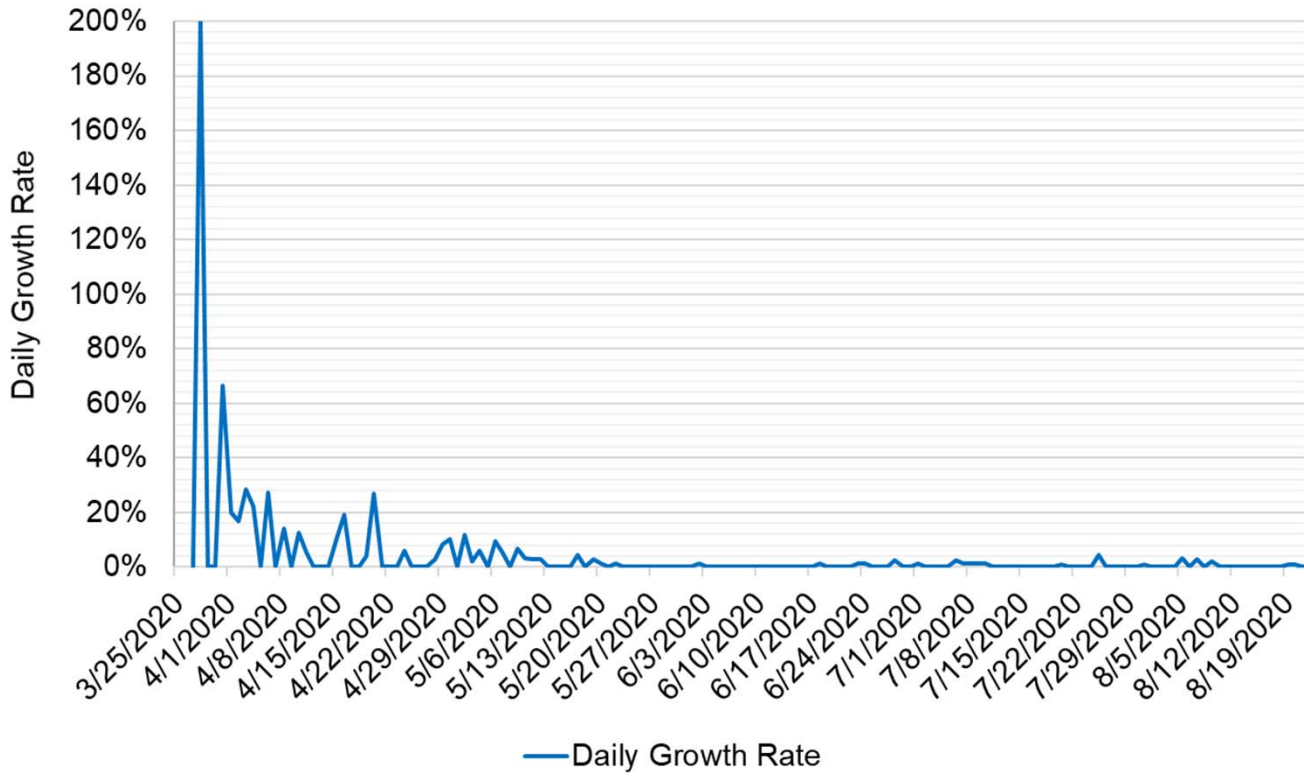
Daily Growth Rate
