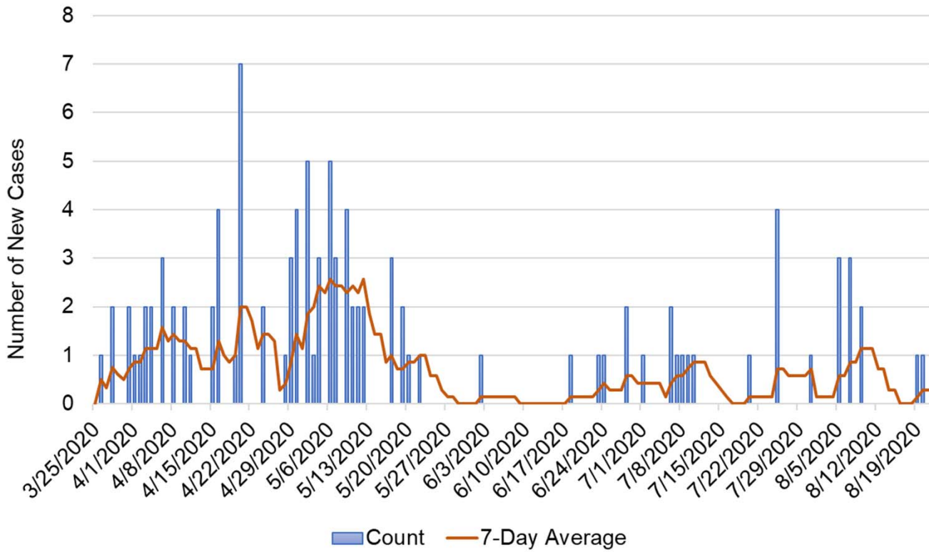
New Cases by Day and Seven-Day Average
